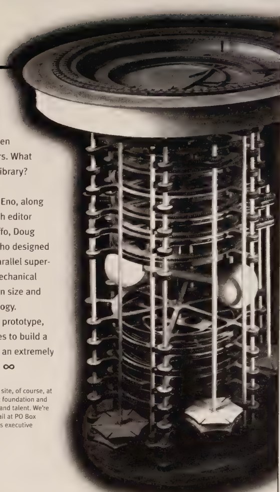
4 - 10,000-year Clock, version 1.0. This is a half-scale model (four feet high) in laser-cut wood of the prototype Clock designed by Danny Hillis. The bottom five rings are a new form of mechanical computer called serial bit adders. The results of their calculations advance the hexagonal Geneva wheels, which drive the top five rings, which translate for the display rings on top. Included in the display are the year (up to 12,000), the positions of the Sun and Moon, Moon phase, the horizon, and the locally visible starfield (which varies subtly over the 25,784-year Precession of the Equinoxes). The two balls in the middle are a torsional (rotating) pendulum. The prototype is being constructed of Monel steel, Invar steel, tungsten carbide, brass, and synthetic sapphire, with diamond coating for low-friction surfaces.
